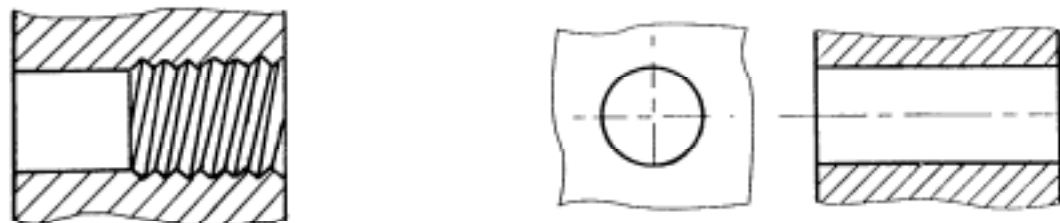
Trou borgne taraudé
